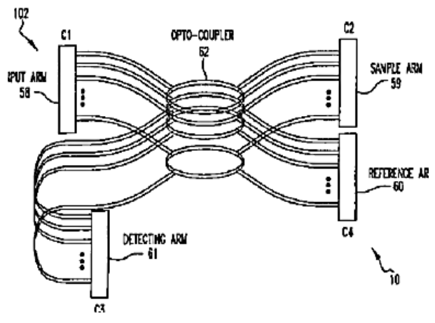
MULTI-PHASE ARRAY OCT SYSTEM
